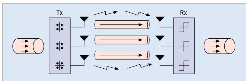
■ Figure 5. A schematic of a spatial multiplexing system.
