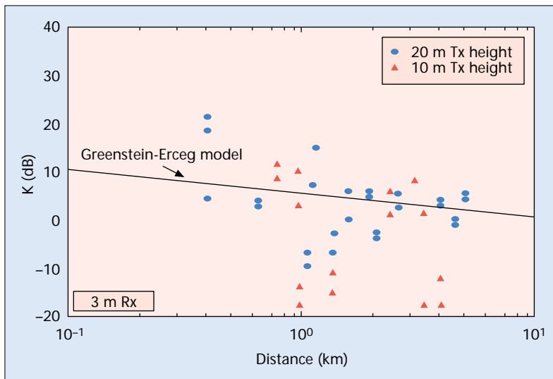
■ Figure 2. K -factor as a function of distance between transmitter and receiver.
