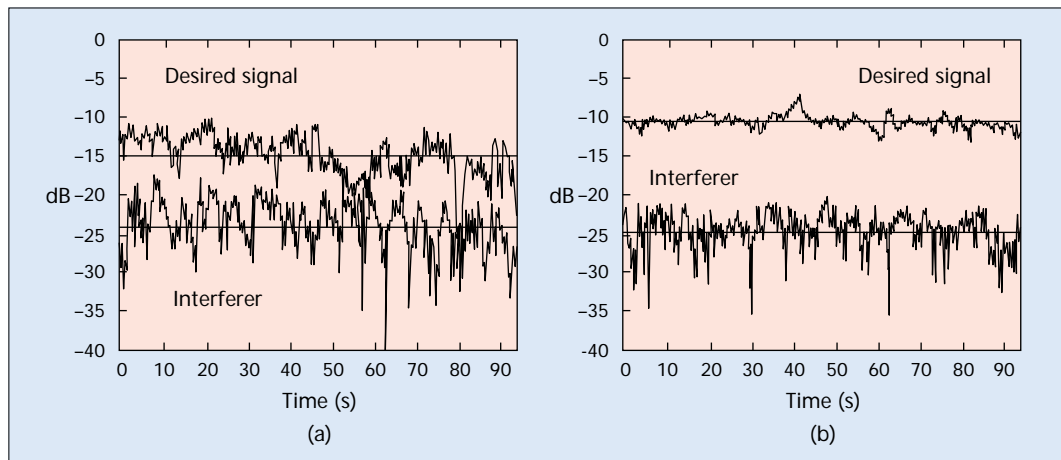
■ Figure 4. Signal and interference levels for an: a) 1-input 1-output; and b) 2-input 3-output system.
