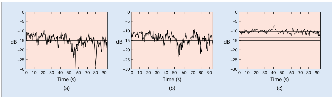
■ Figure 3. Signal level at the receiver of: a) a 1-input 1-output; b) a 1-input 2-output; and c) a 2-input 3-output system.
